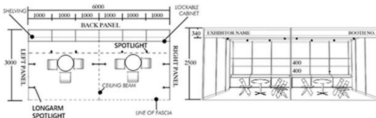
PLAN VIEW
