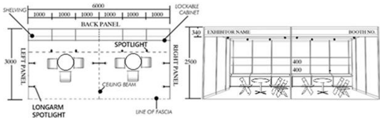
PLAN VIEW
